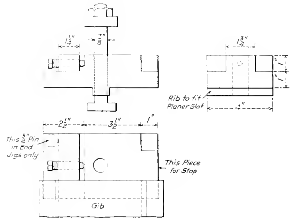
Jig for Planing Crosshead Shoes
